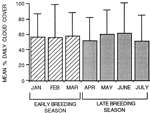
FIG. 3. Cloud cover patterns during the 1973–1975 Common Amakihi breeding seasons at 2130 m elevation on the southwestern slope of Mauna Kea, Hawaii. Vertical lines are ± one SD.
